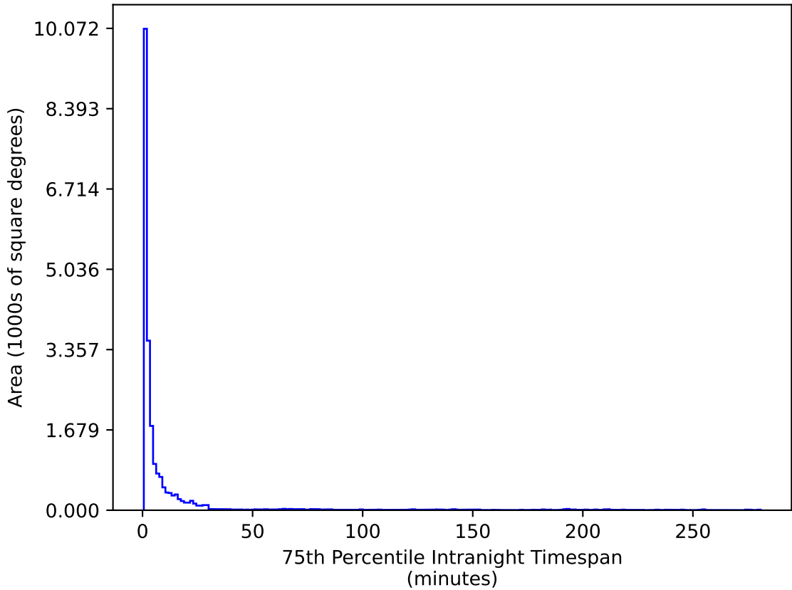
noroll_mjdp180_v3.4_10yrs All sky u band: 75th Percentile Intranight Timespan
