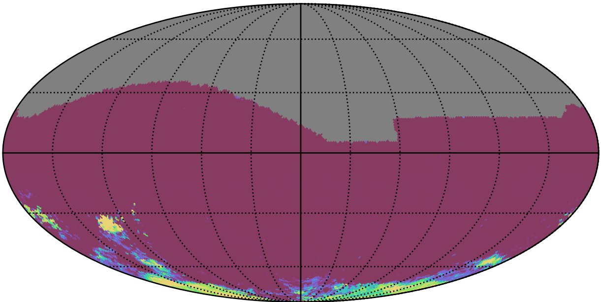
noroll_mjdp180_v3.4_10yrs All sky ri bands: 75th Percentile Intranight Timespan
