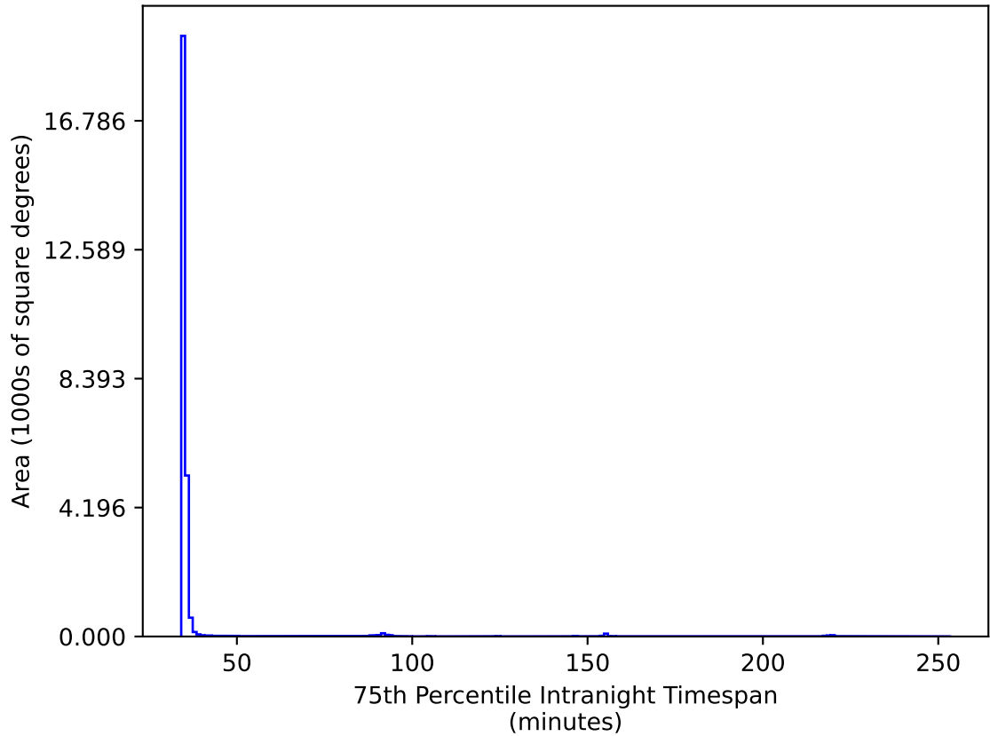
noroll_mjdp180_v3.4_10yrs All sky ri bands: 75th Percentile Intranight Timespan
