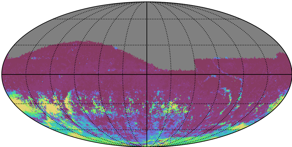
noroll_mjdp180_v3.4_10yrs All sky r band: 75th Percentile Intranight Timespan
