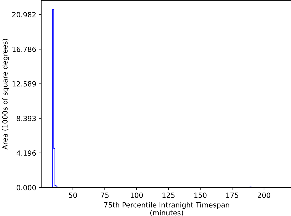
noroll_mjdp180_v3.4_10yrs All sky iz bands: 75th Percentile Intranight Timespan
