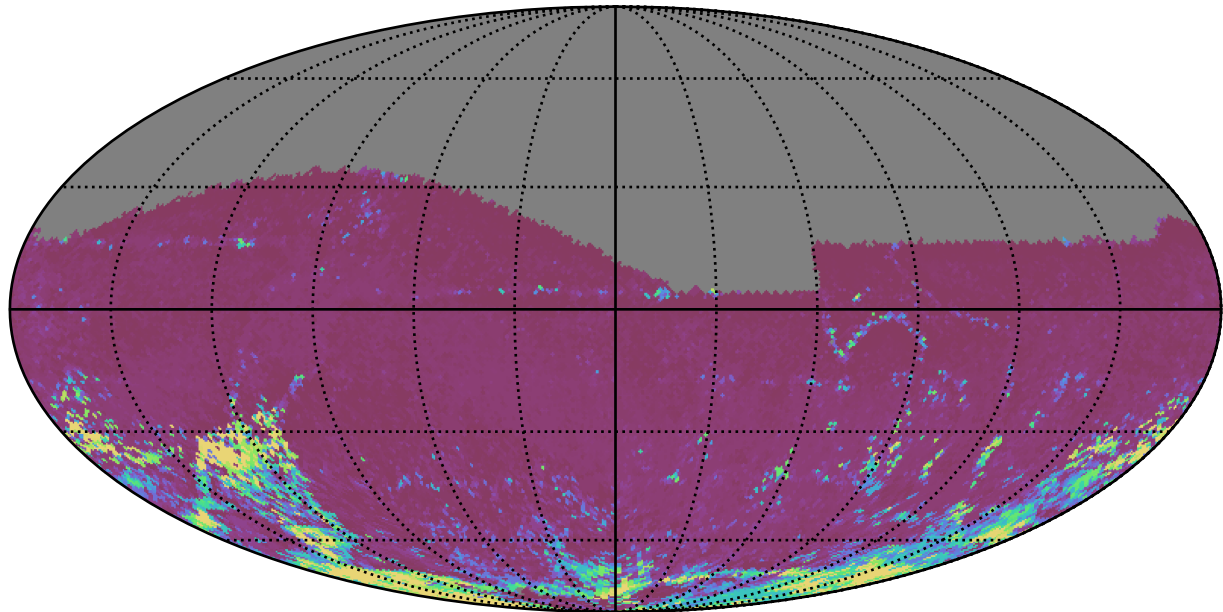
noroll_mjdp180_v3.4_10yrs All sky i band: 75th Percentile Intranight Timespan
