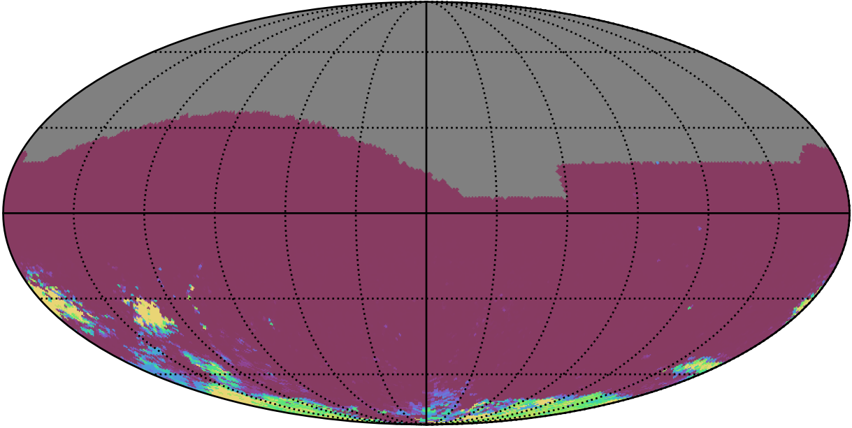
noroll_mjdp180_v3.4_10yrs All sky gr bands: 75th Percentile Intranight Timespan
