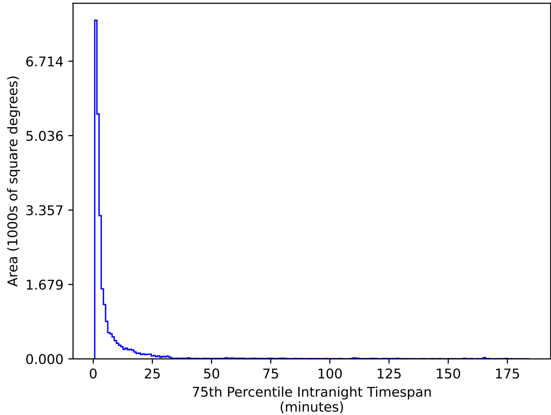
noroll_mjdp180_v3.4_10yrs All sky g band: 75th Percentile Intranight Timespan
