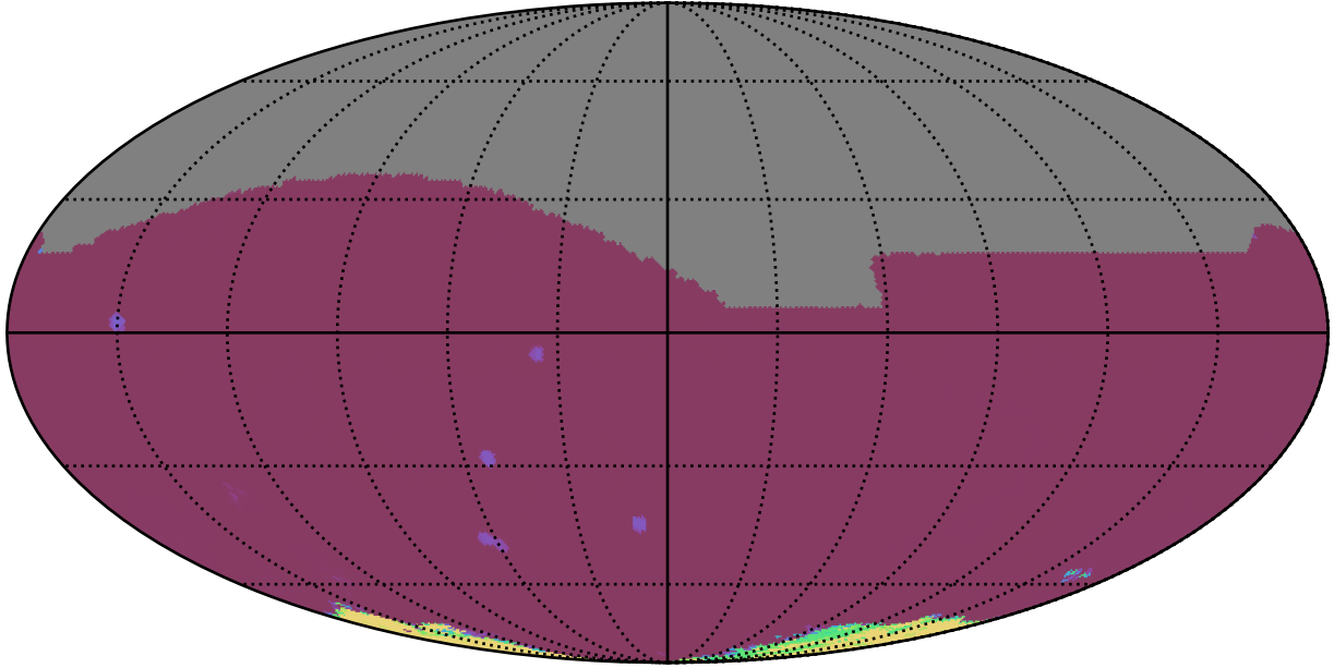
noroll_mjdp180_v3.4_10yrs All sky all bands: 75th Percentile Intranight Timespan
