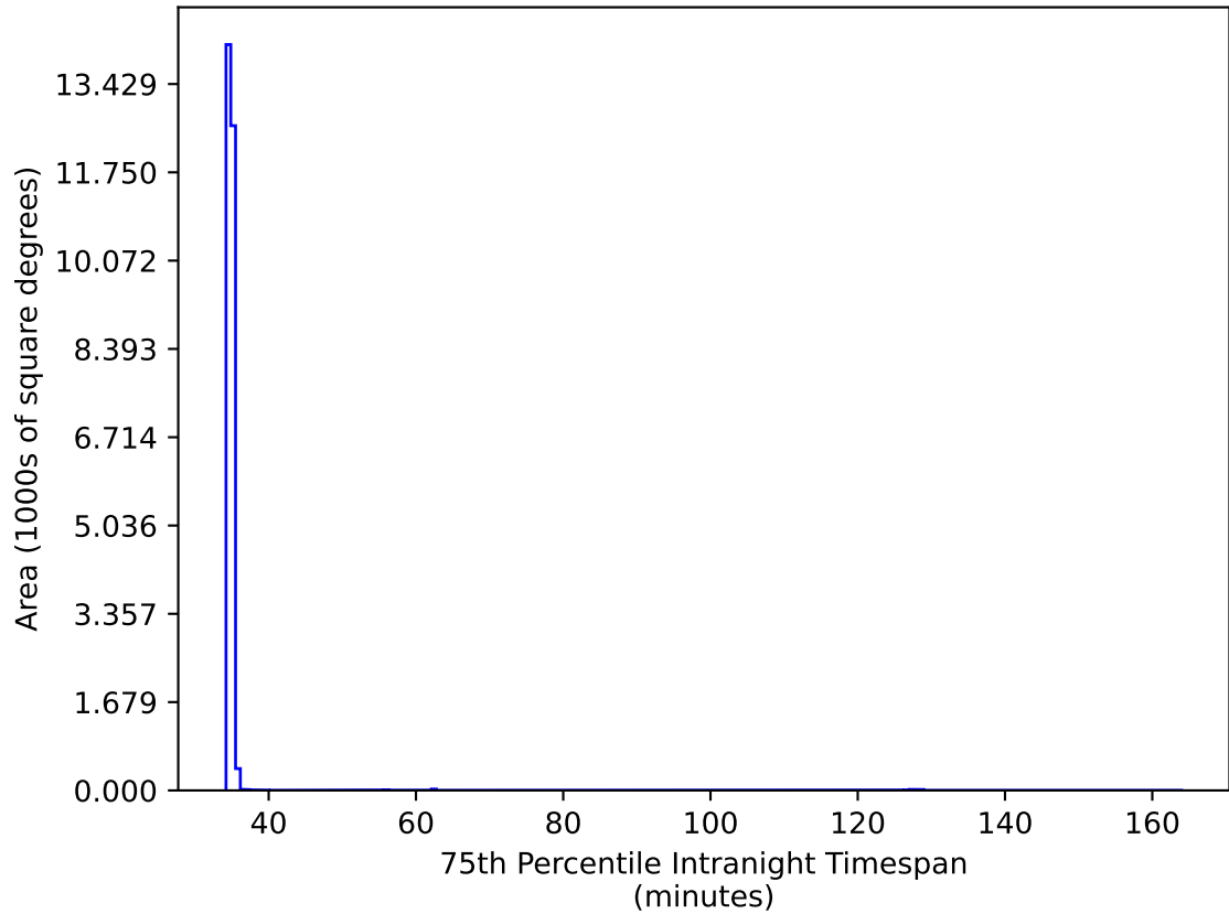
noroll_mjdp180_v3.4_10yrs All sky all bands: 75th Percentile Intranight Timespan
