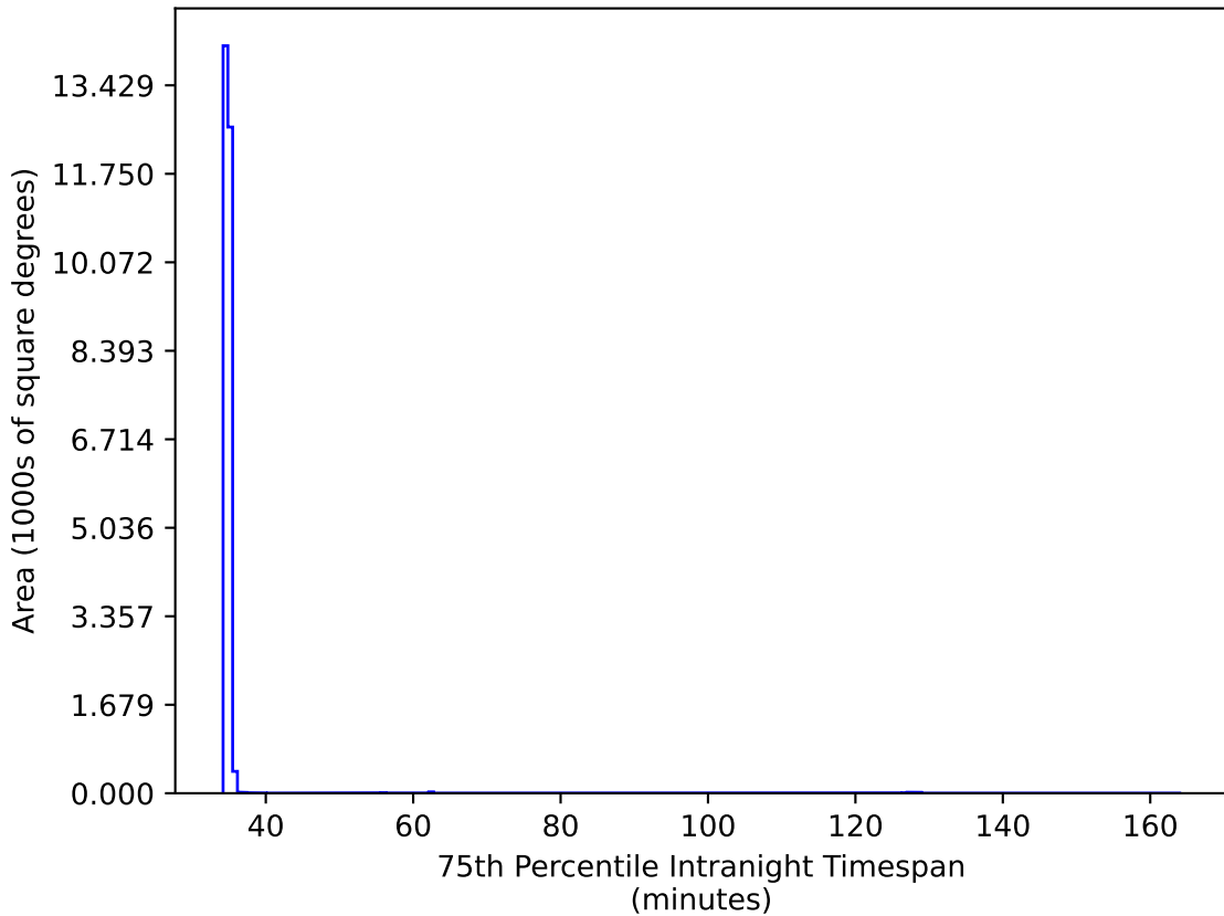
noroll_mjdp180_v3.4_10yrs All sky: 75th Percentile Intranight Timespan
