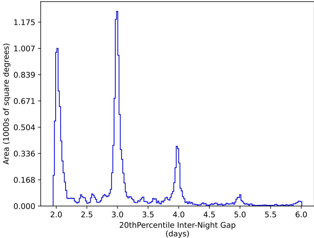
noroll_mjdp180_v3.4_10yrs WFD y band: 20thPercentile Inter-Night Gap
