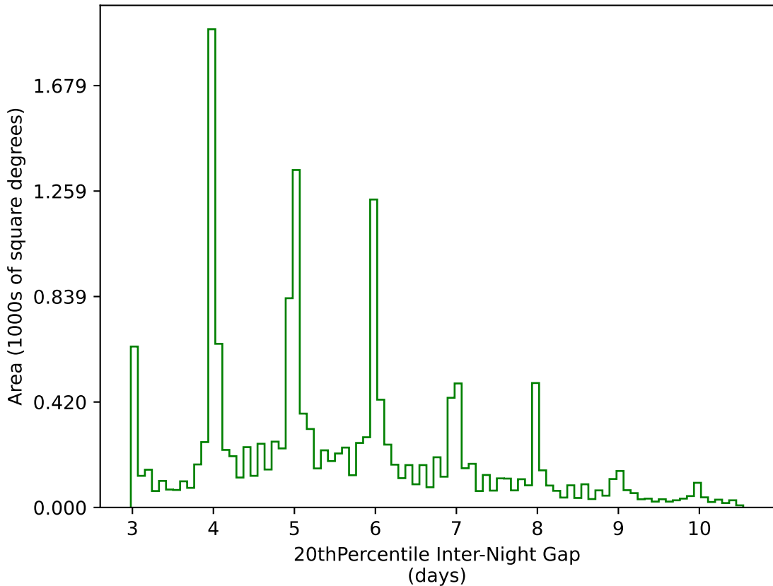
noroll_mjdp180_v3.4_10yrs WFD g band: 20thPercentile Inter-Night Gap
