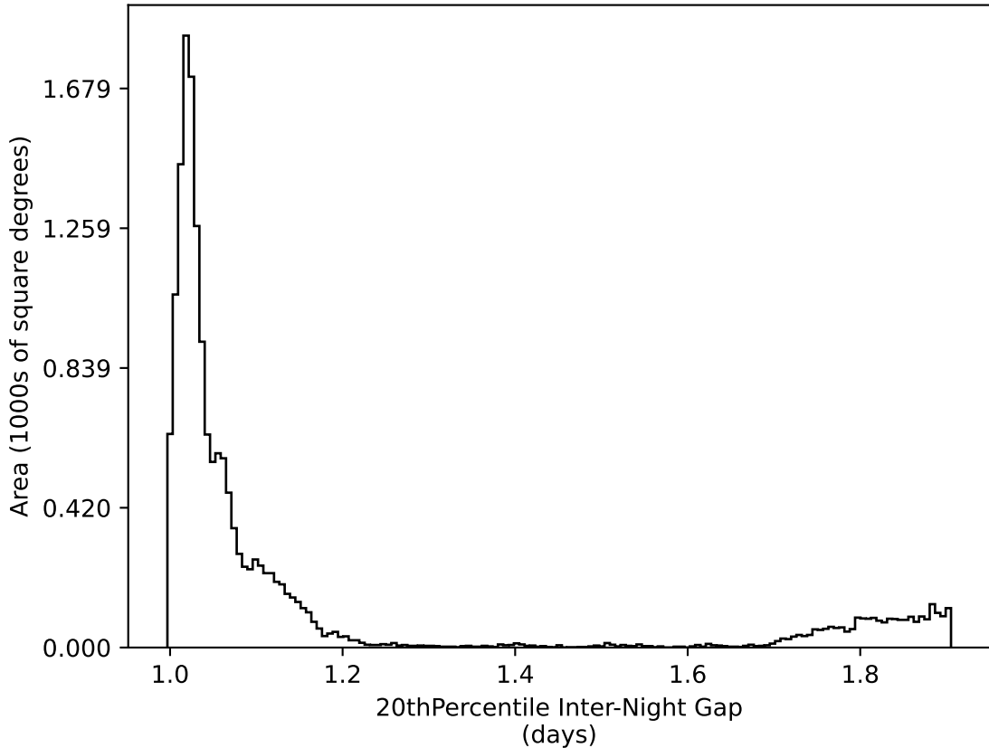
noroll_mjdp180_v3.4_10yrs WFD all bands: 20thPercentile Inter-Night Gap
