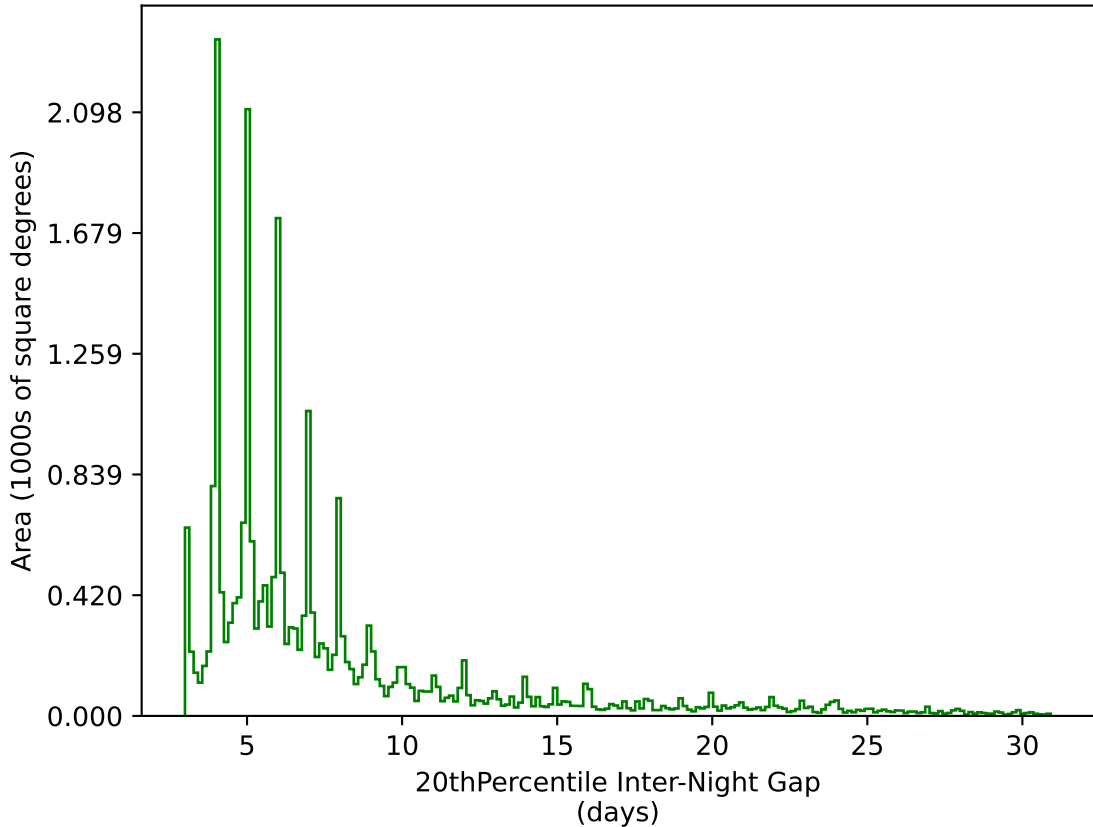
noroll_mjdp180_v3.4_10yrs All sky g band: 20thPercentile Inter-Night Gap
