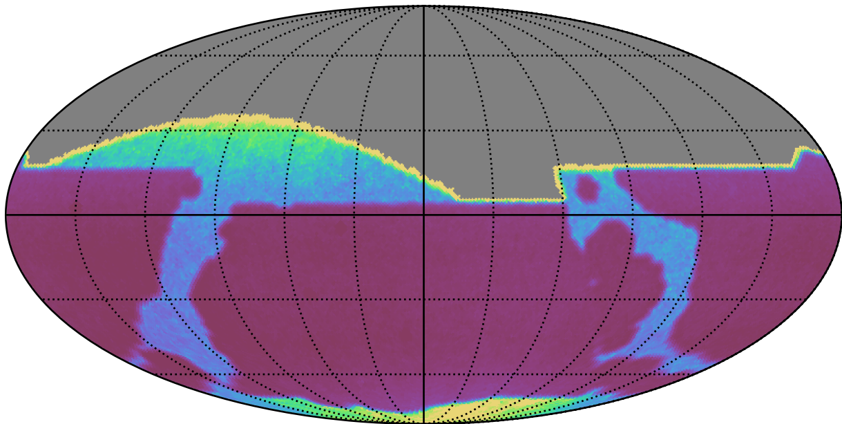
noroll_mjdp180_v3.4_10yrs : properMotion
