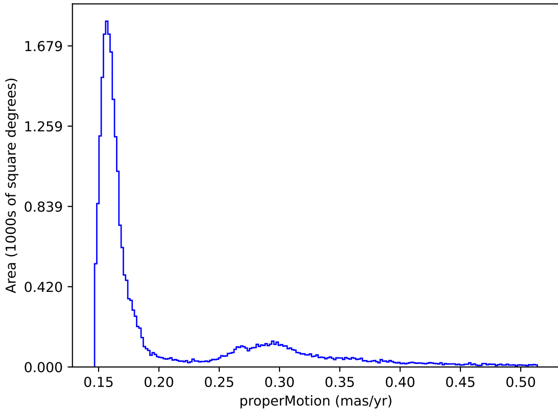
noroll_mjdp180_v3.4_10yrs : properMotion
