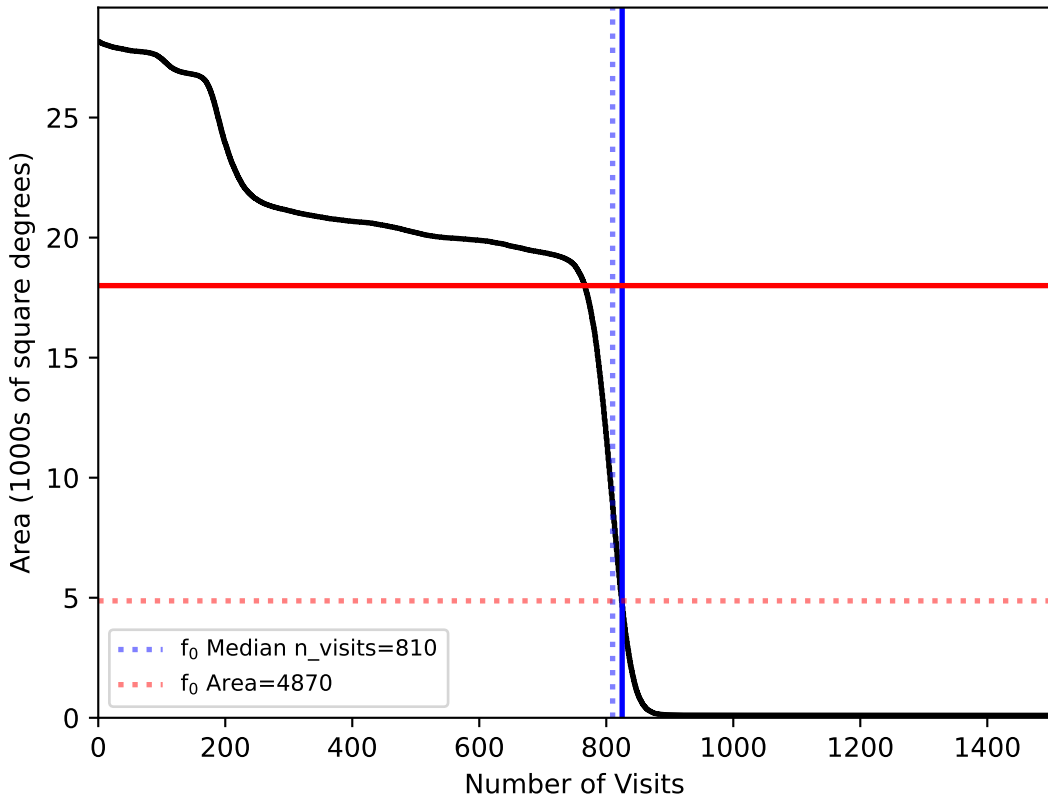
noroll_mjdp180_v3.4_10yrs : f0
