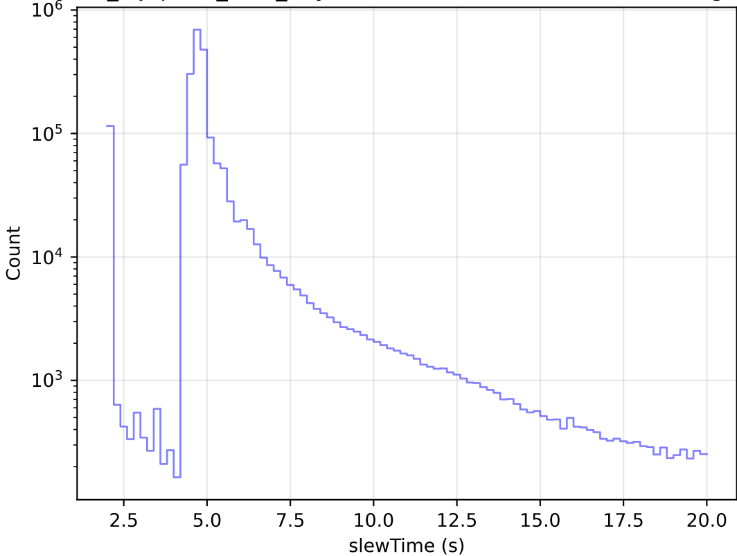
noroll_mjdp180_v3.4_10yrs All visits: Zoom Slew Time Histogram
