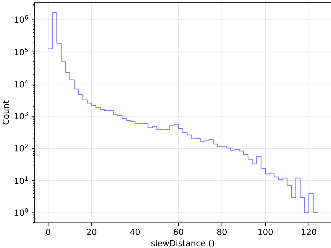
noroll_mjdp180_v3.4_10yrs All visits: Slew Distance Histogram
