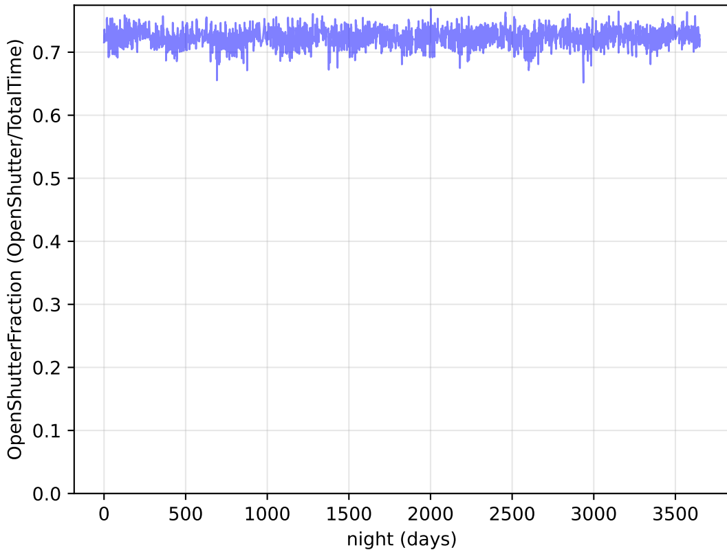
noroll_mjdp180_v3.4_10yrs : OpenShutterFraction
