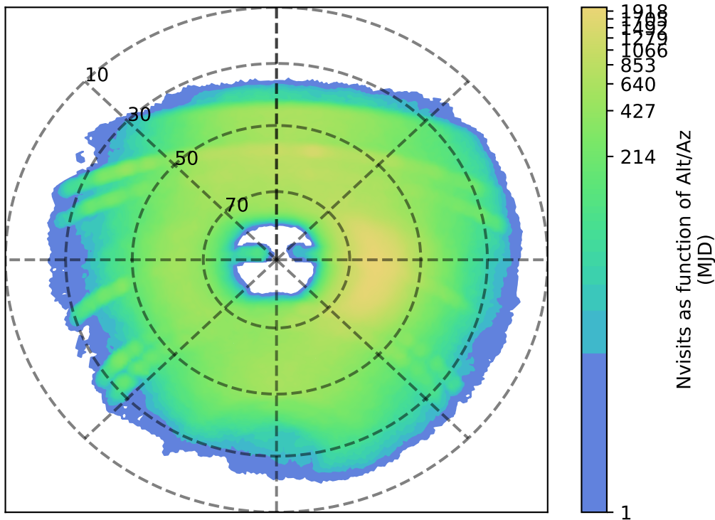
noroll_mjdp180_v3.4_10yrs y: Nvisits as function of Alt/Az
