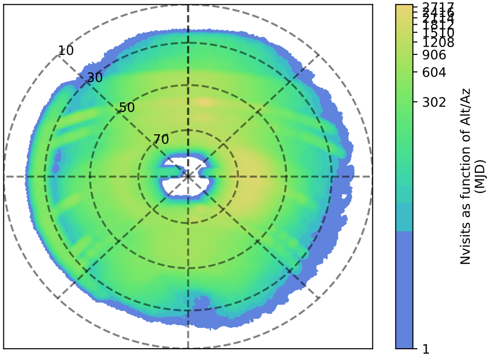
noroll_mjdp180_v3.4_10yrs r: Nvisits as function of Alt/Az
