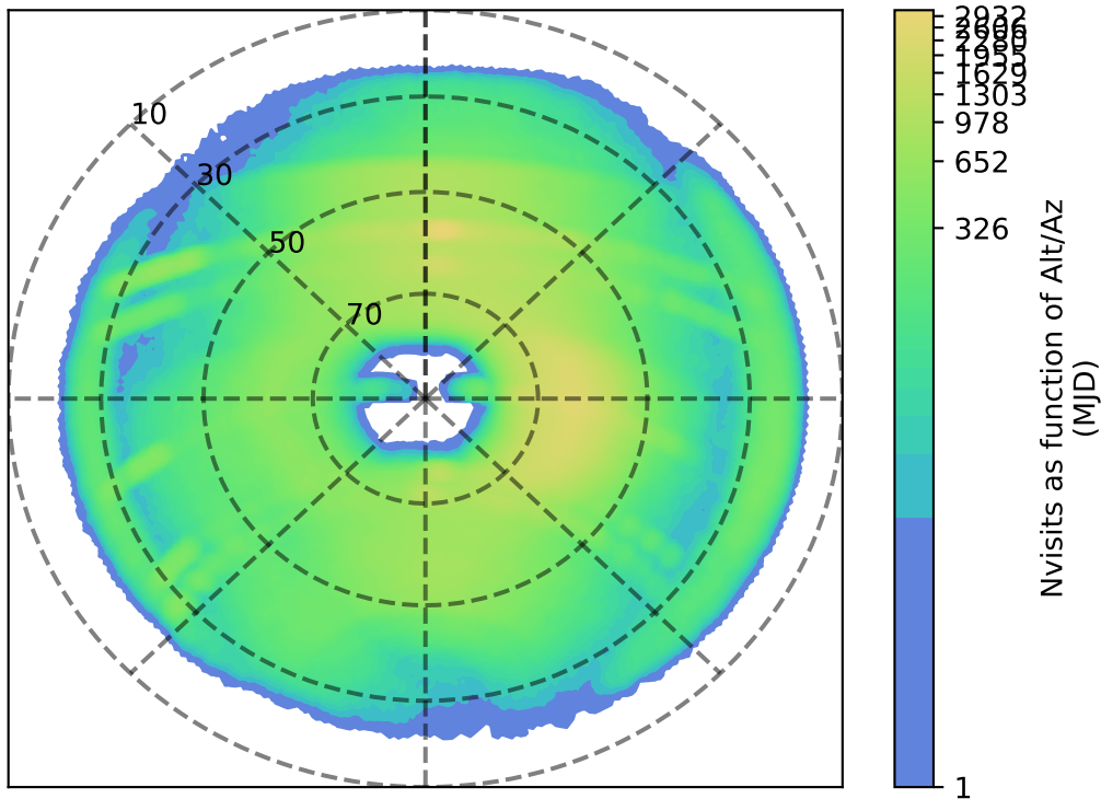
noroll_mjdp180_v3.4_10yrs i: Nvisits as function of Alt/Az
