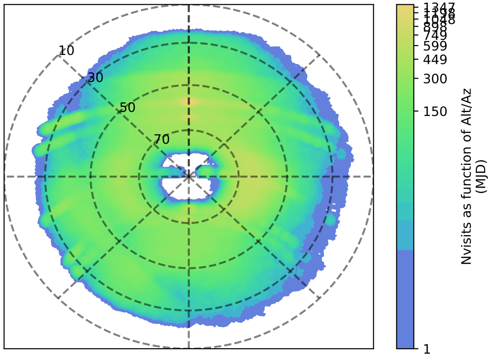
noroll_mjdp180_v3.4_10yrs g: Nvisits as function of Alt/Az
