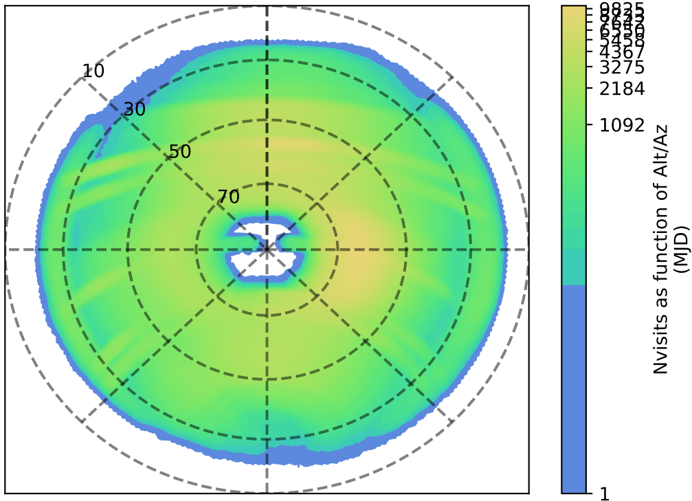
noroll_mjdp180_v3.4_10yrs : Nvisits as function of Alt/Az
