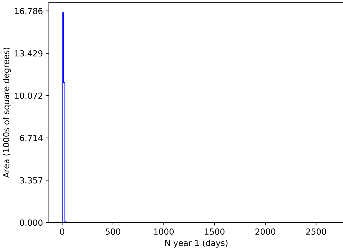
noroll_mjdp180_v3.4_10yrs z and night < 365: N year 1
