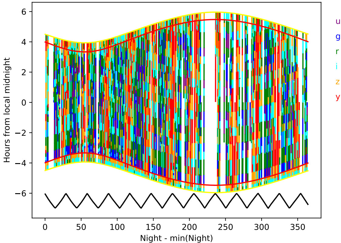
noroll_mjdp180_v3.4_10yrs year 9-10: Hourglass
