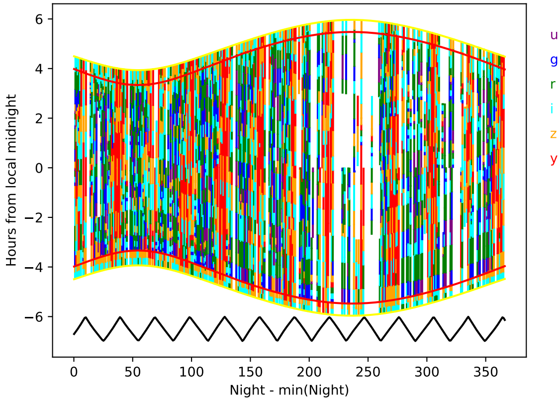
noroll_mjdp180_v3.4_10yrs year 8-9: Hourglass
