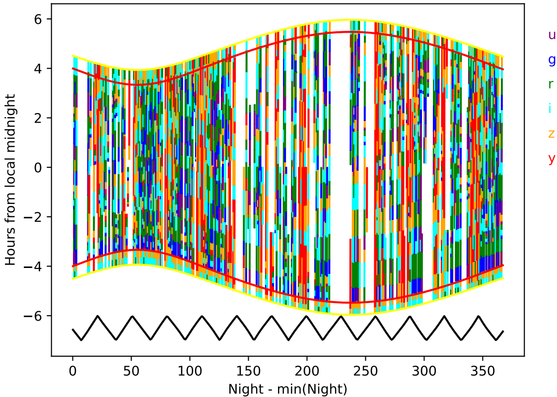
noroll_mjdp180_v3.4_10yrs year 7-8: Hourglass
