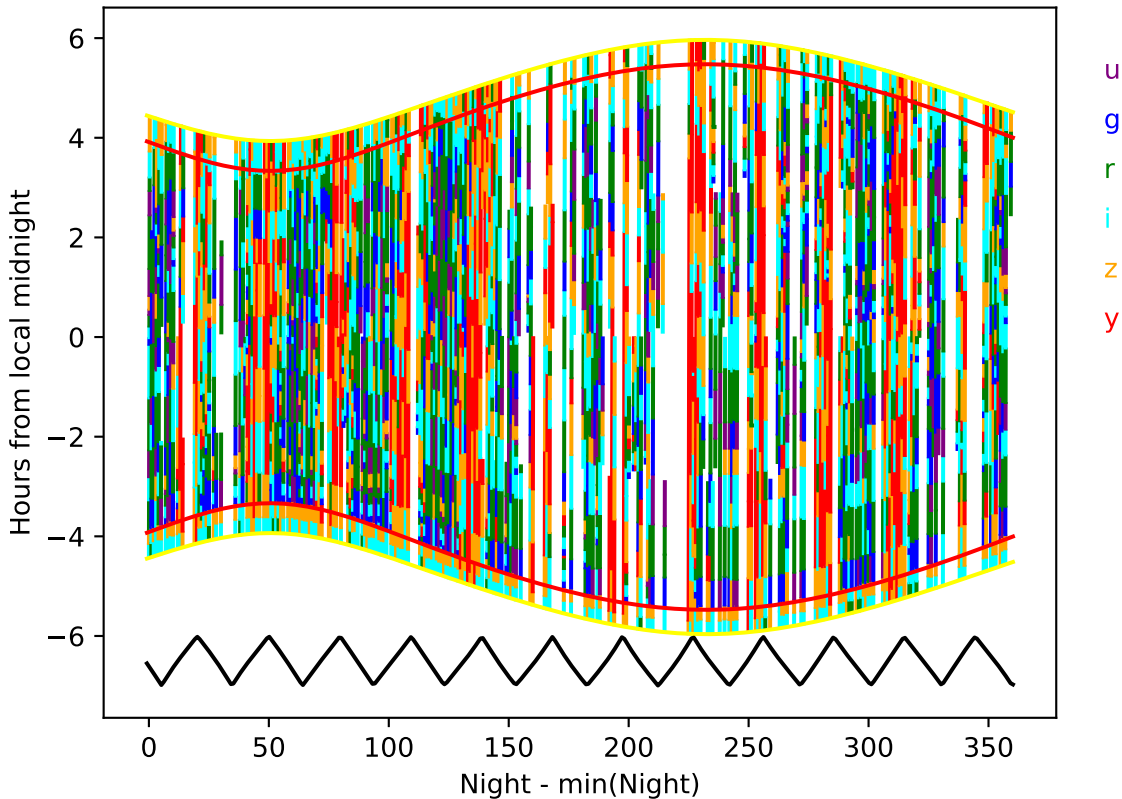
noroll_mjdp180_v3.4_10yrs year 4-5: Hourglass
