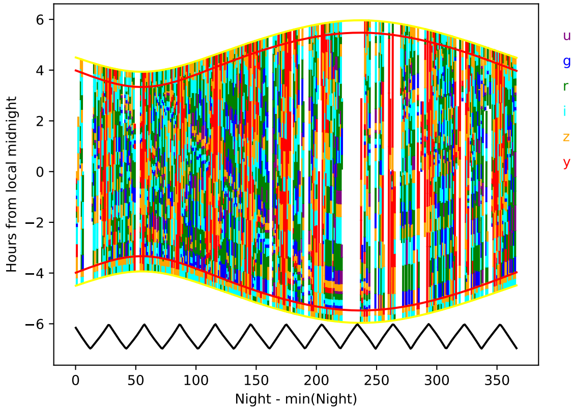
noroll_mjdp180_v3.4_10yrs year 1-2: Hourglass
