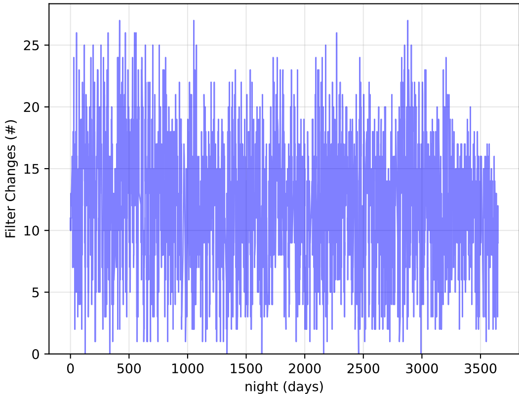
noroll_mjdp180_v3.4_10yrs : Filter Changes
