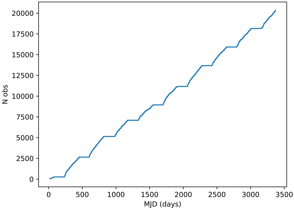
noroll_mjdp180_v3.4_10yrs note like DD:ELAISS1%: Cumulative
