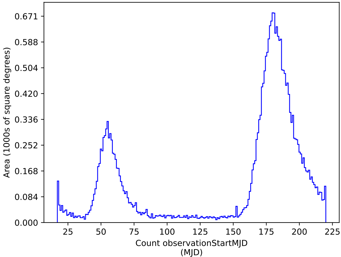
noroll_mjdp180_v3.4_10yrs r: Count observationStartMJD
