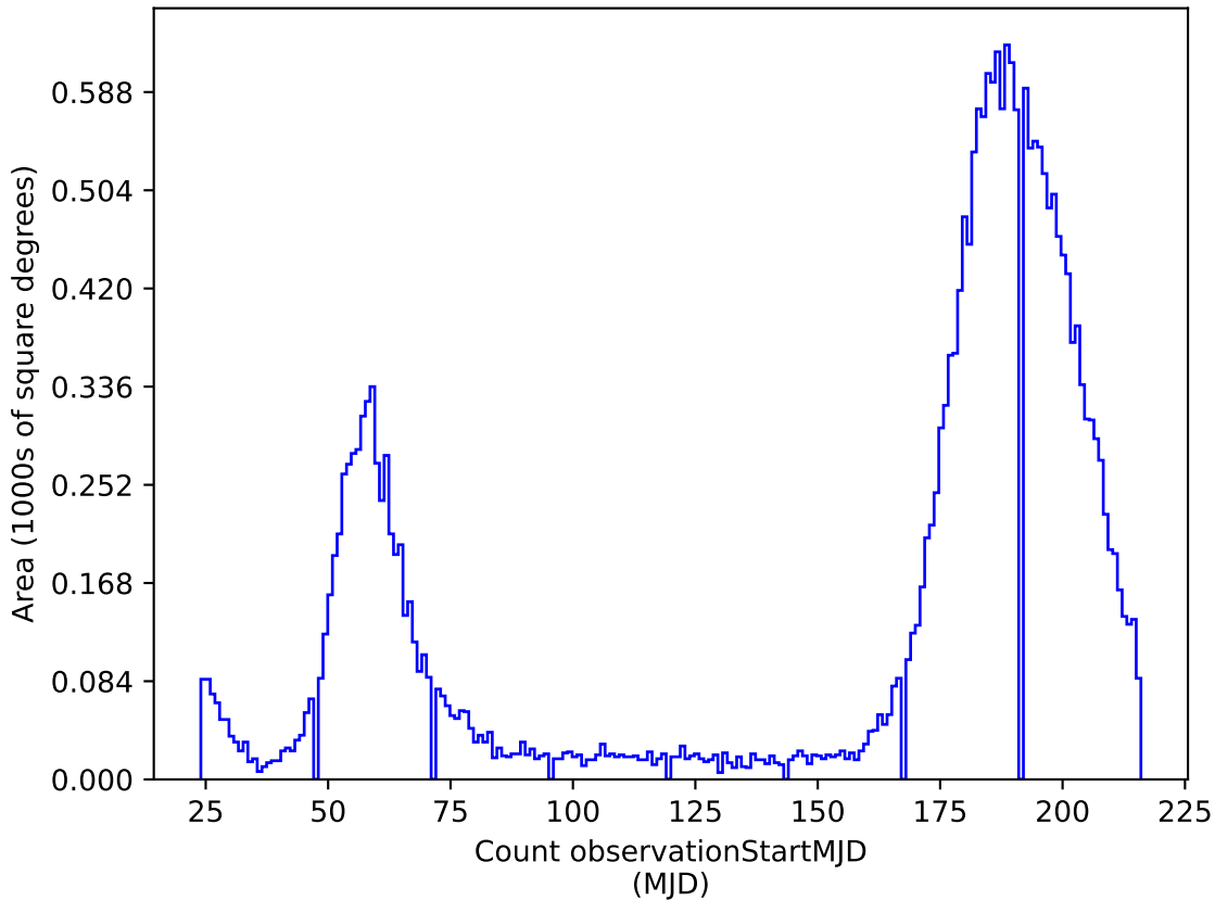
noroll_mjdp180_v3.4_10yrs i: Count observationStartMJD
