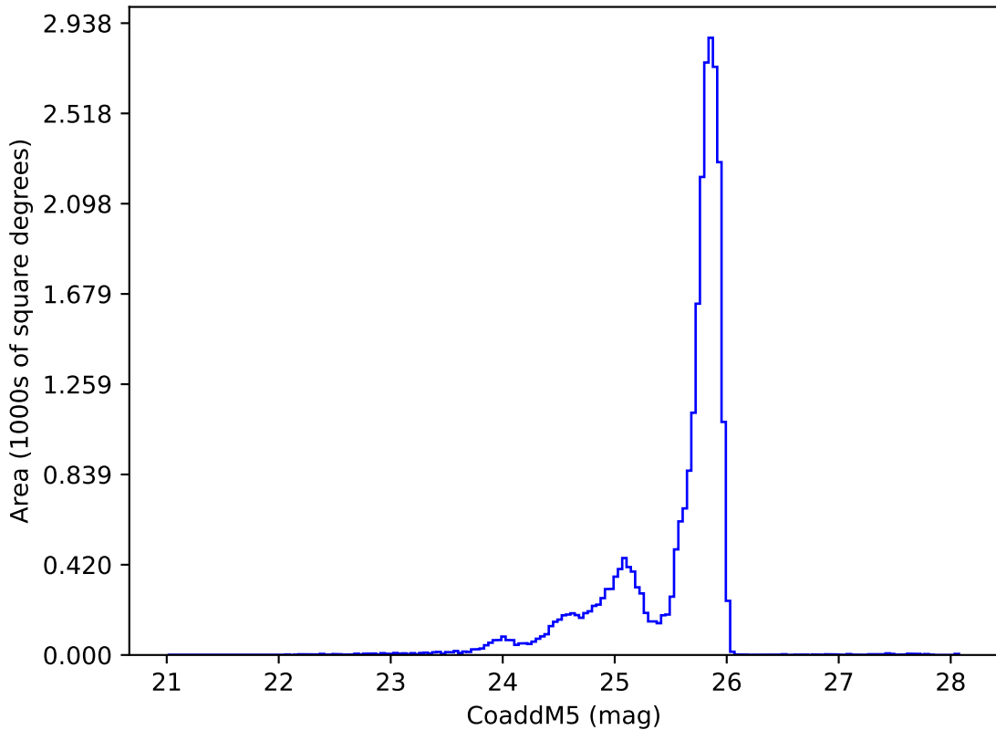
noroll_mjdp180_v3.4_10yrs z: CoaddM5
