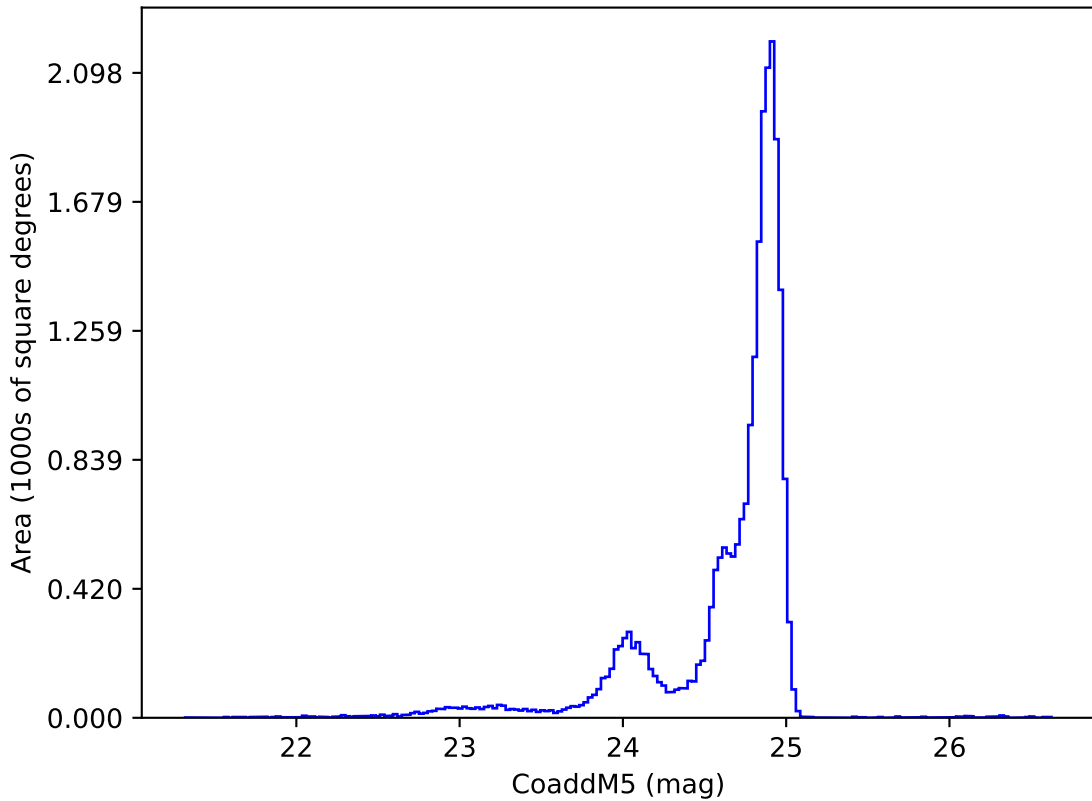
noroll_mjdp180_v3.4_10yrs y: CoaddM5
