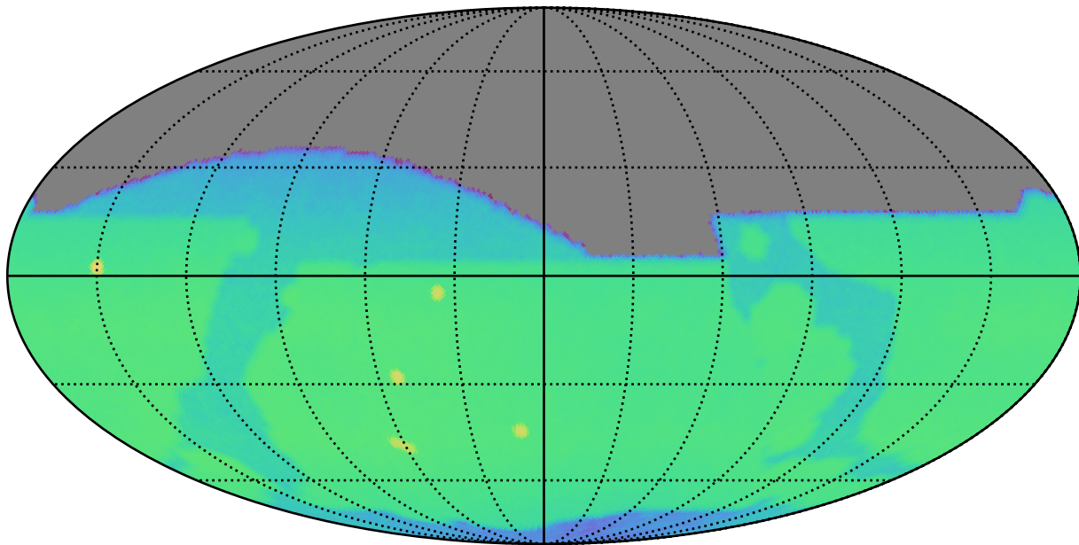
noroll_mjdp180_v3.4_10yrs r: CoaddM5
