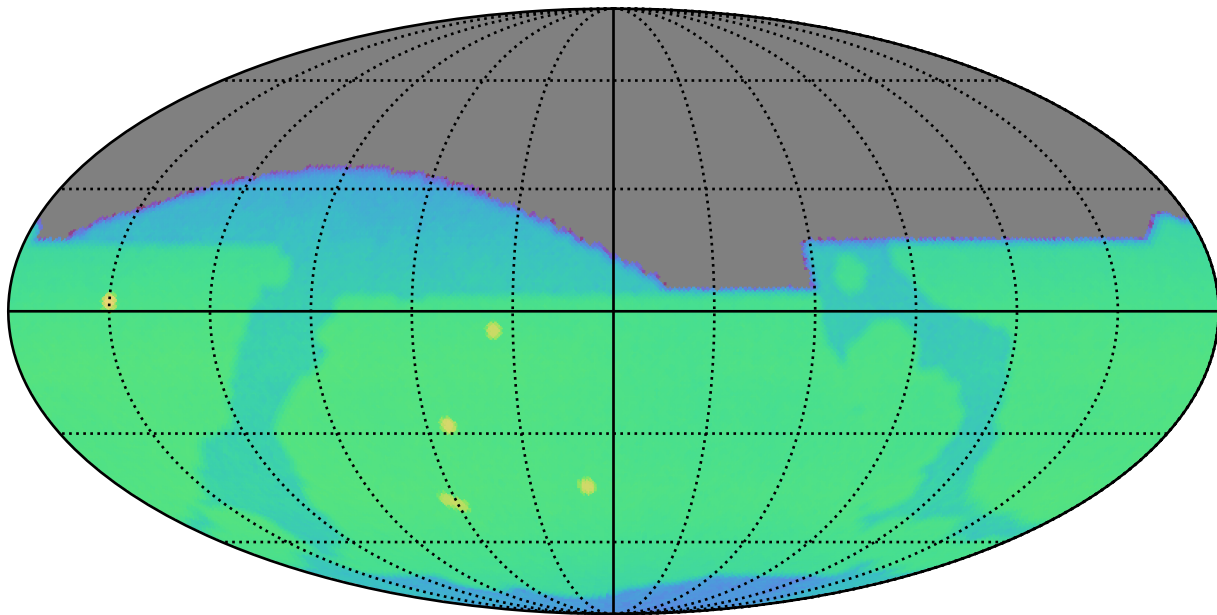
noroll_mjdp180_v3.4_10yrs i: CoaddM5
