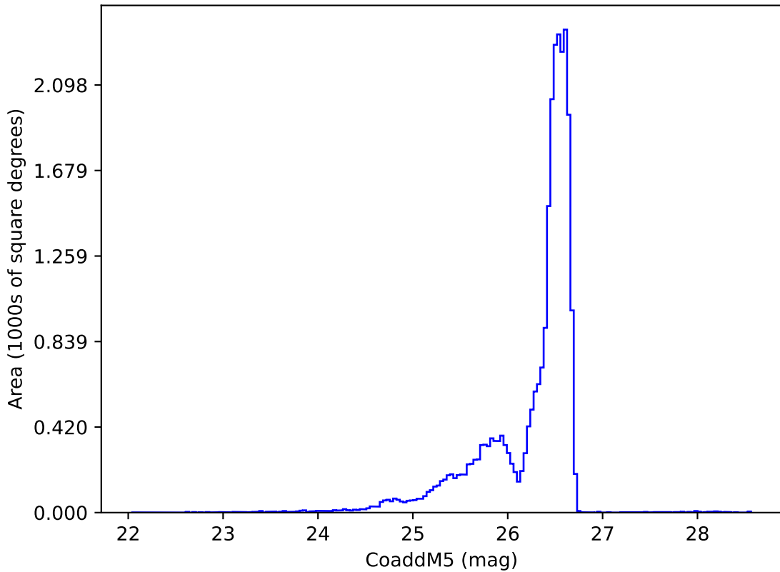
noroll_mjdp180_v3.4_10yrs i: CoaddM5
