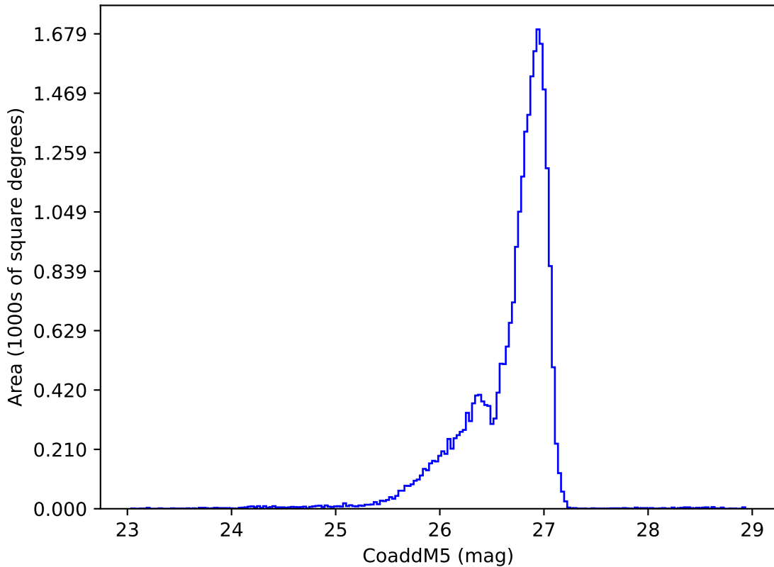
noroll_mjdp180_v3.4_10yrs g: CoaddM5
