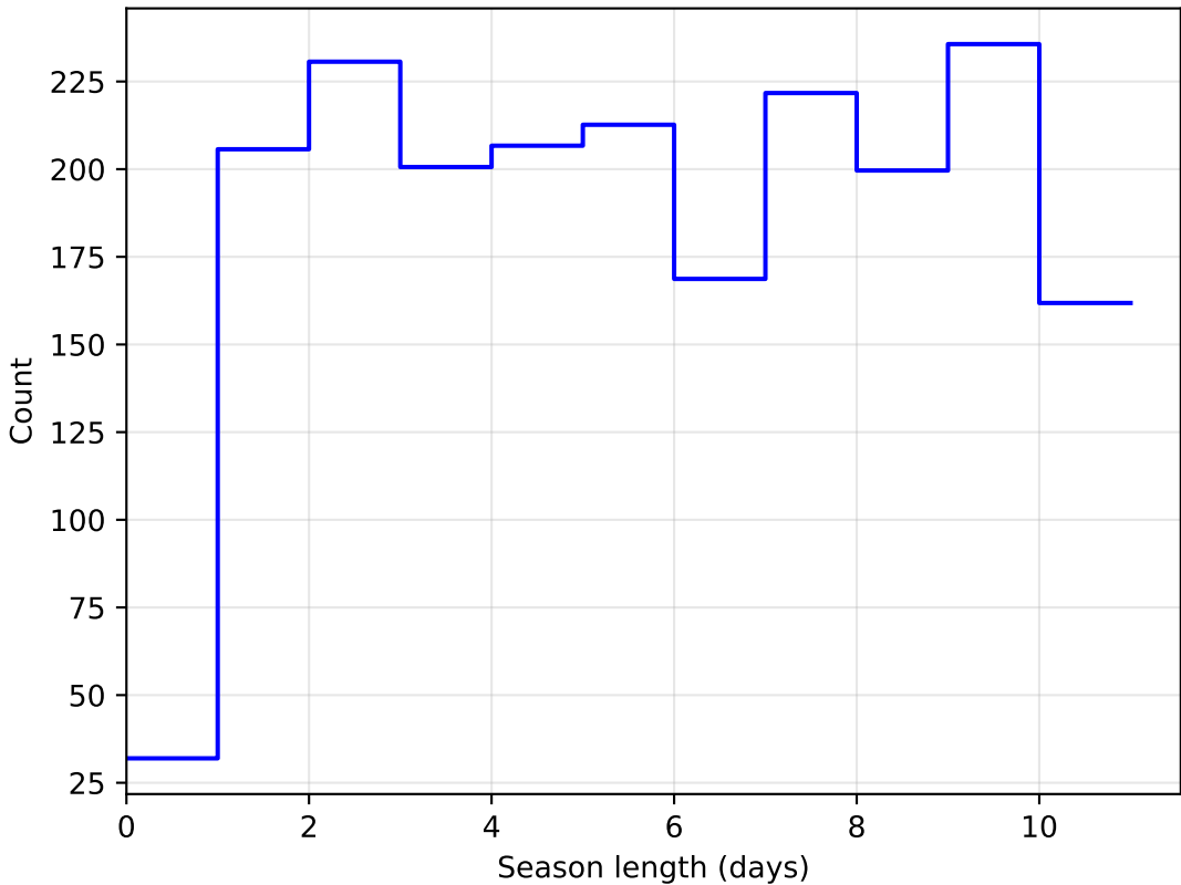
noroll_mjdp180_v3.4_10yrs DD:WFD all bands: SeasonLength
