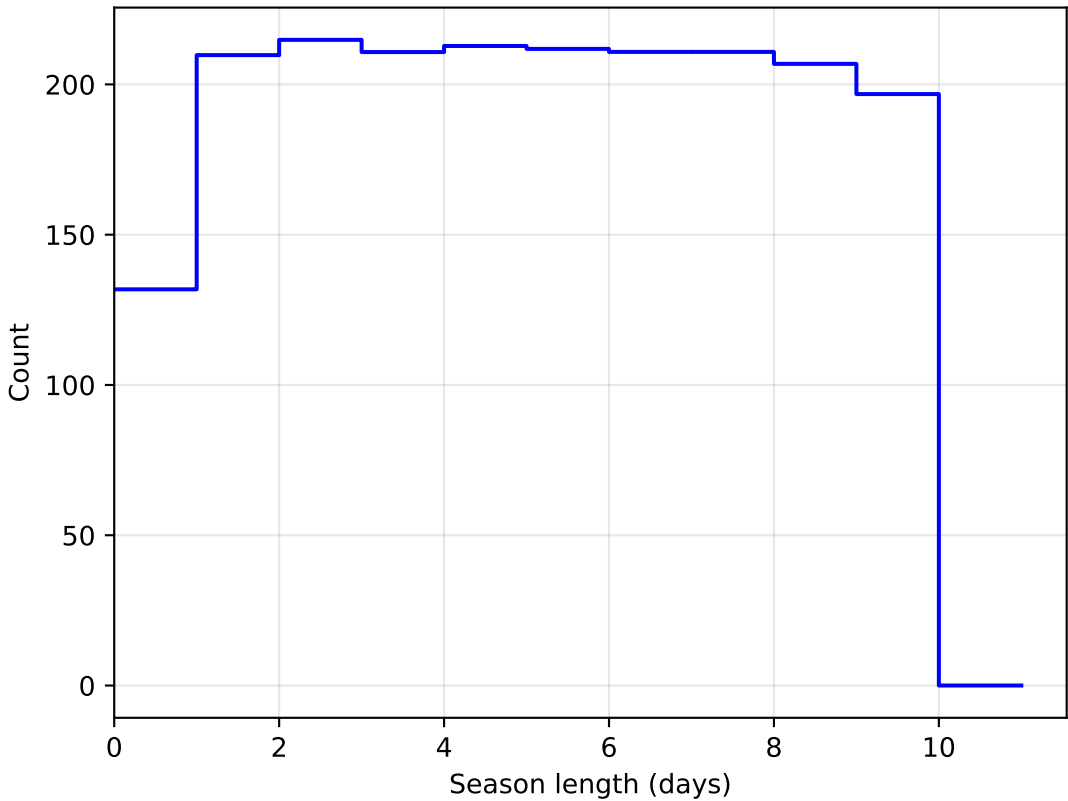
noroll_mjdp180_v3.4_10yrs DD:EDFS all bands: SeasonLength
