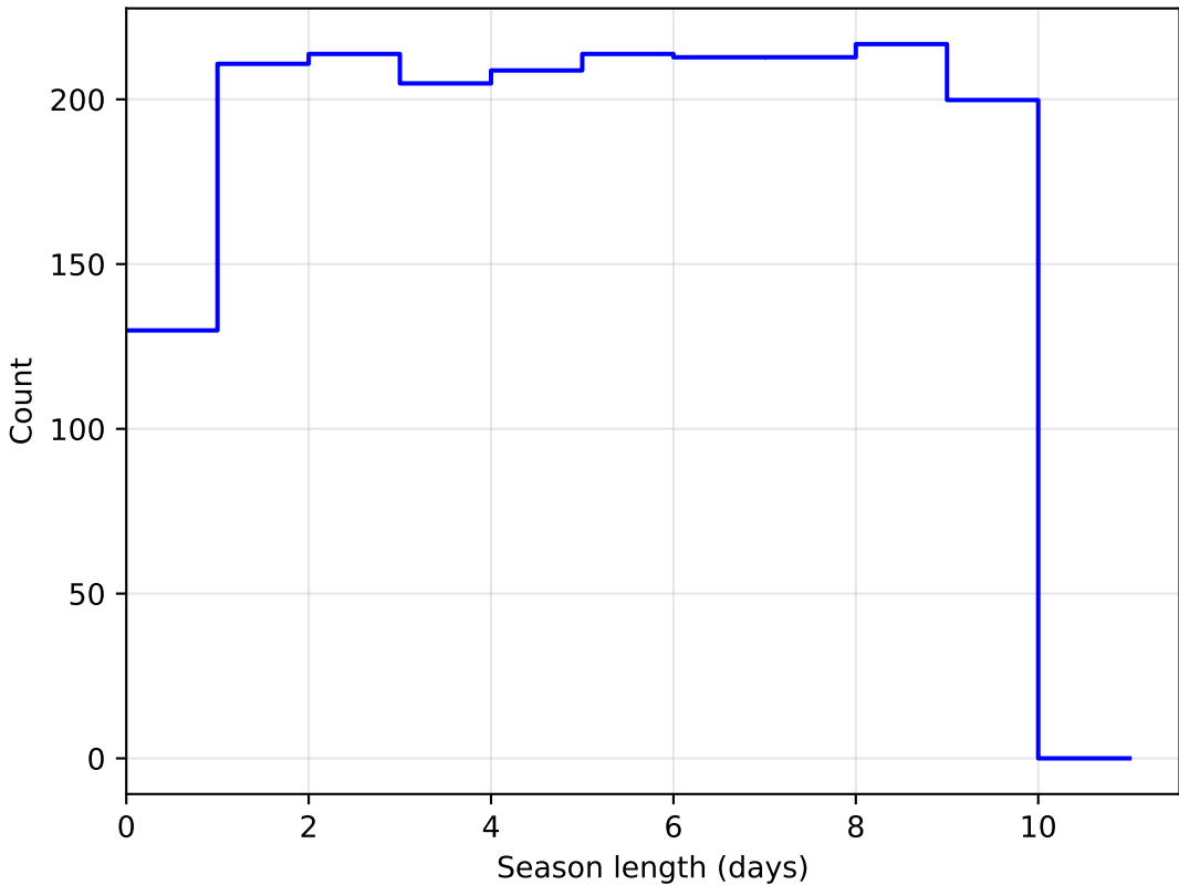
noroll_mjdp180_v3.4_10yrs DD:ECDFS all bands: SeasonLength
