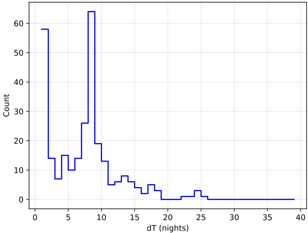
noroll_mjdp180_v3.4_10yrs all bands: DD:XMM_LSS Delta Nights Histogram
