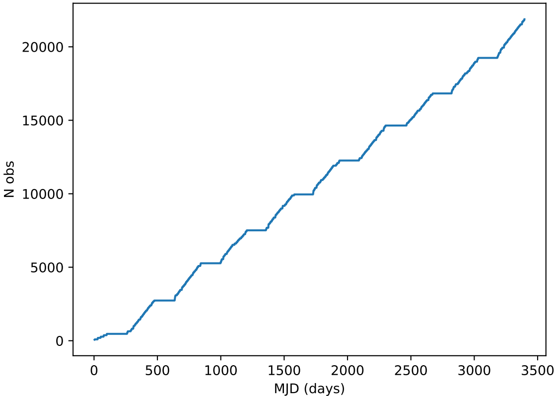
noroll_mjdp180_v3.4_10yrs all bands: DD:XMM_LSS Cumulative NVisits
