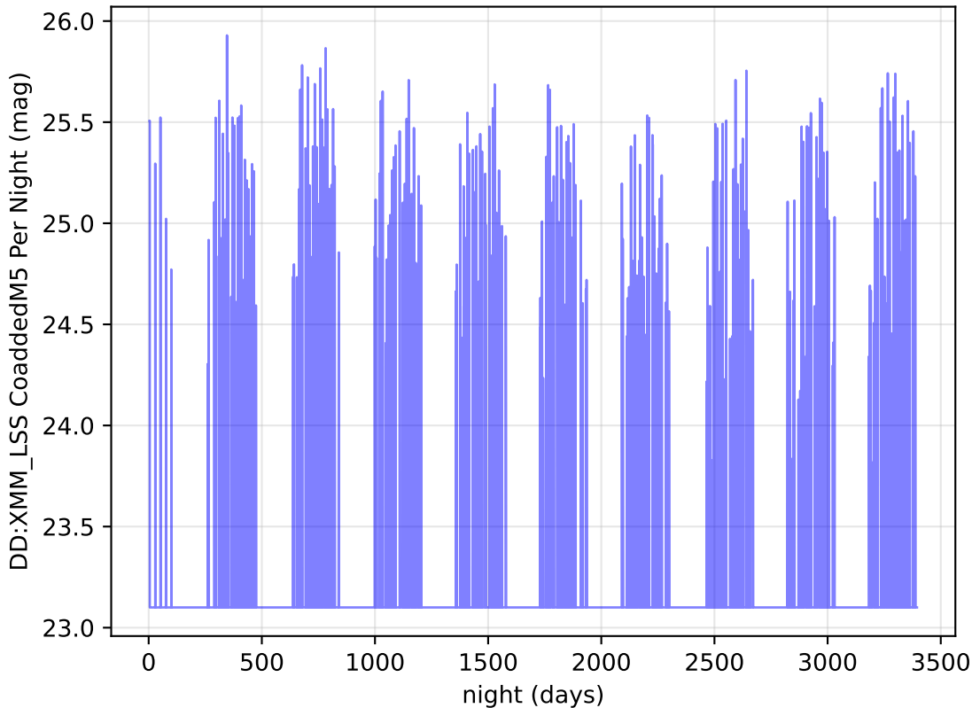
noroll_mjdp180_v3.4_10yrs i band: DD:XMM_LSS CoaddedM5 Per Night
