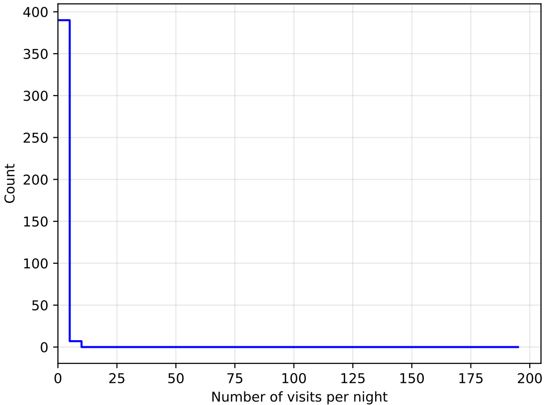
noroll_mjdp180_v3.4_10yrs all bands: DD:WFD NVisitsPerNight
