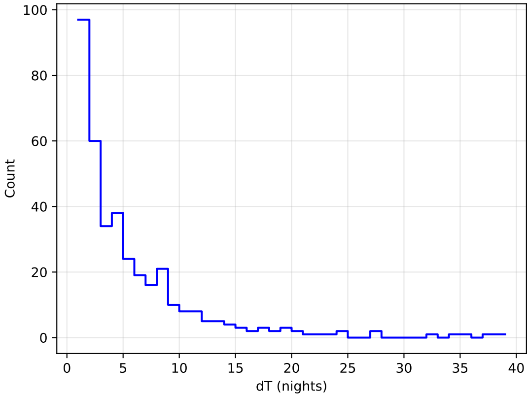
noroll_mjdp180_v3.4_10yrs all bands: DD:WFD Delta Nights Histogram
